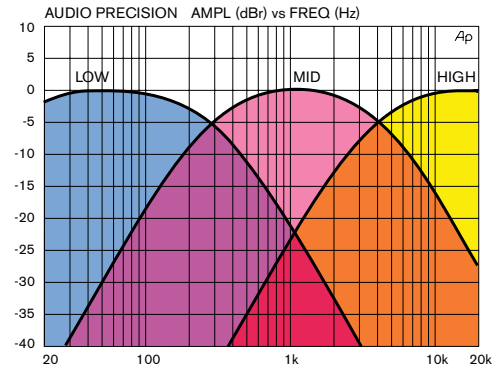
This chart shows the response of each Low, Mid and High tone control when the other two are set to OFF (full cut).
