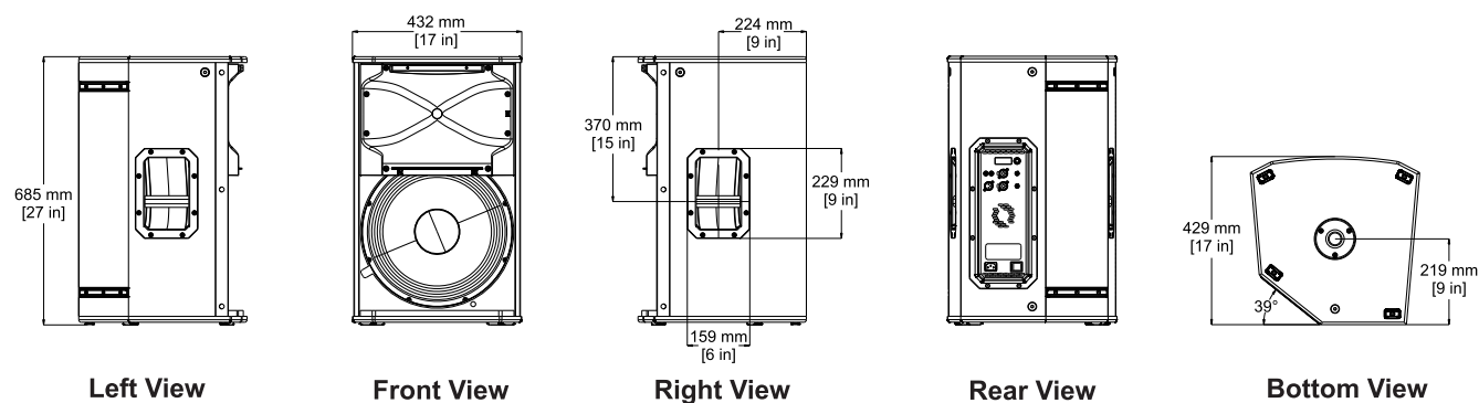
Figure 3.2: EKV-15P dimensions
