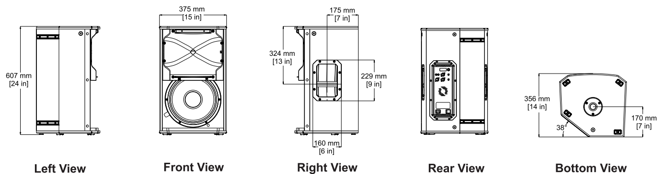
Figure 3.1: EKV-12P dimensions
